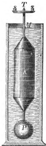
Aréometer.
